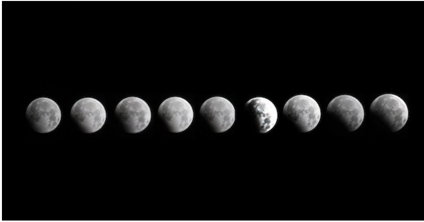
Image of the change of moonlight when a lunar eclipse occurs in Hanoi.
